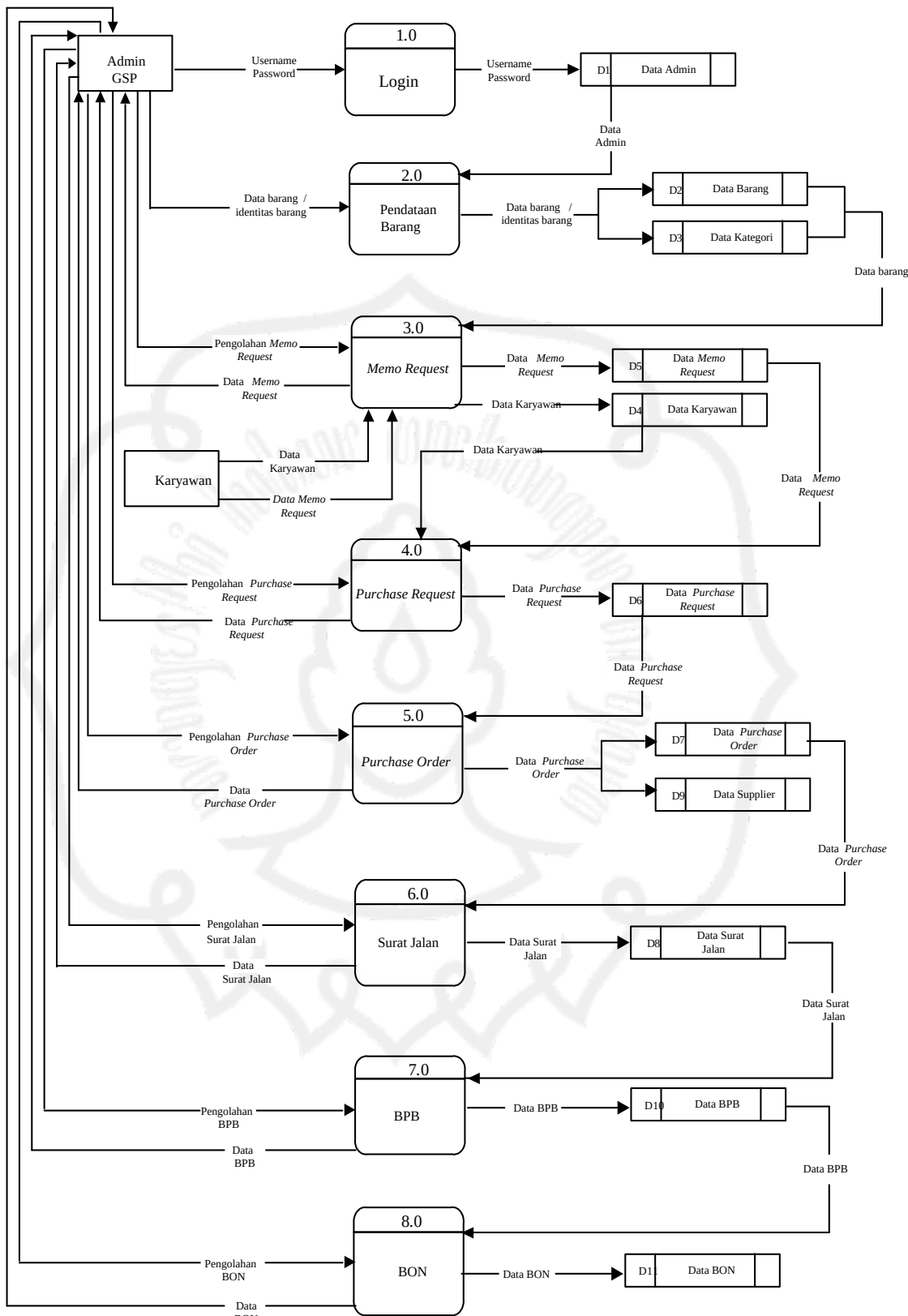
Gambar 7. DFD level 0
